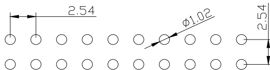
PCB LAYOUT
